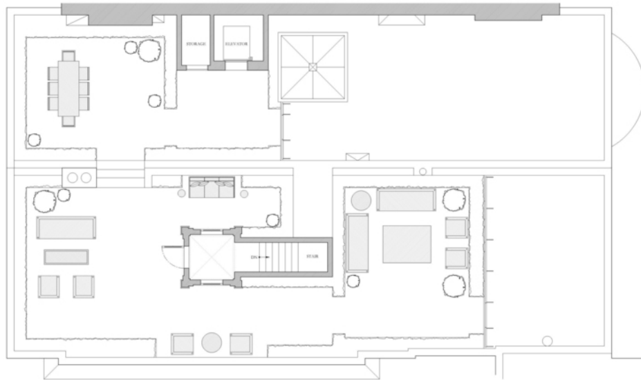
PPA PROPOSED FOURTH FLOOR PLAN
